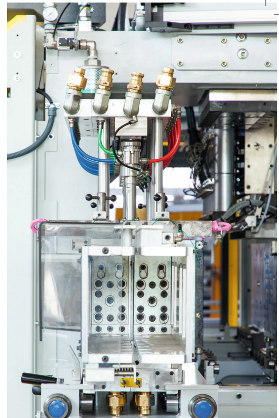
Centered blowing station on the blow mould with take-out device
