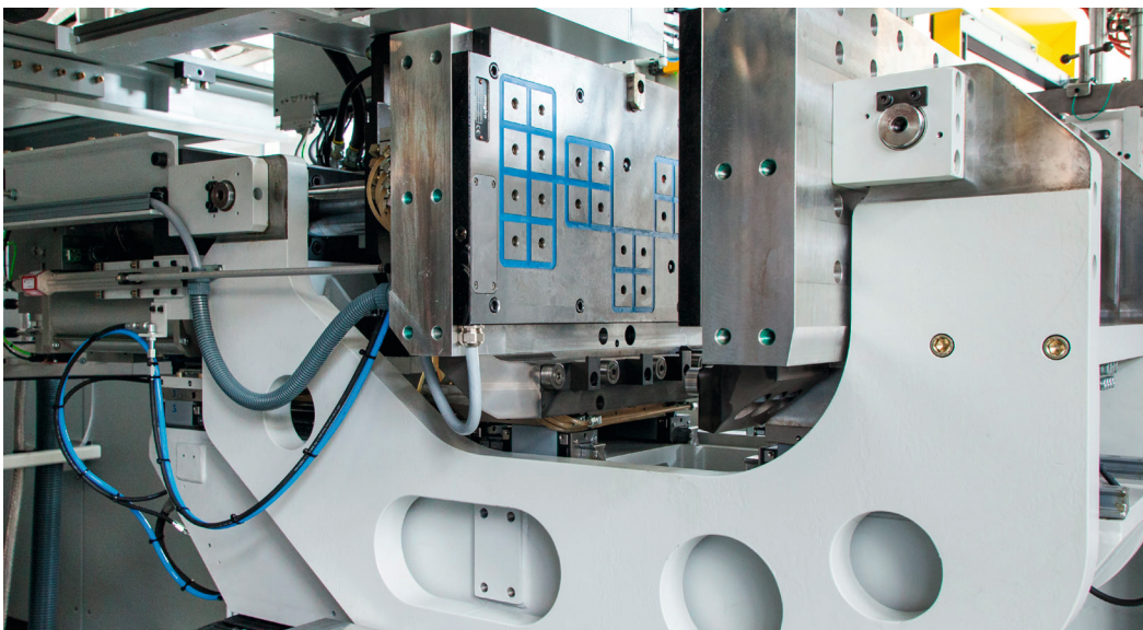
Magnetic mounting plates in the patented C-frame clamping unit
